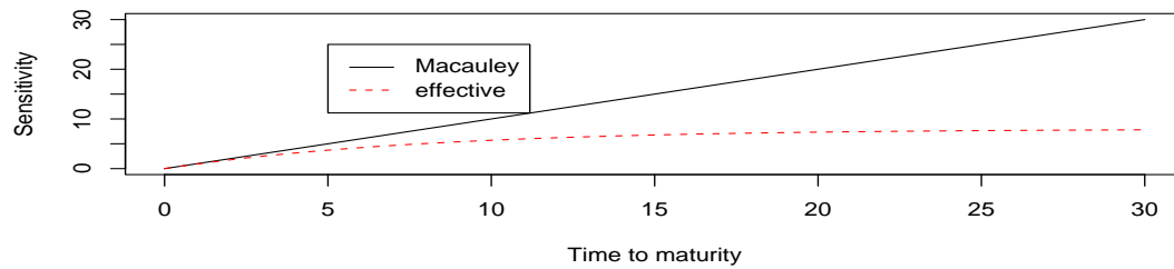
Sensitivity of zero-coupon yields to an interest shock
