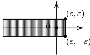
Figure 1. The \varepsilon -thickened half-line B_\varepsilon .
